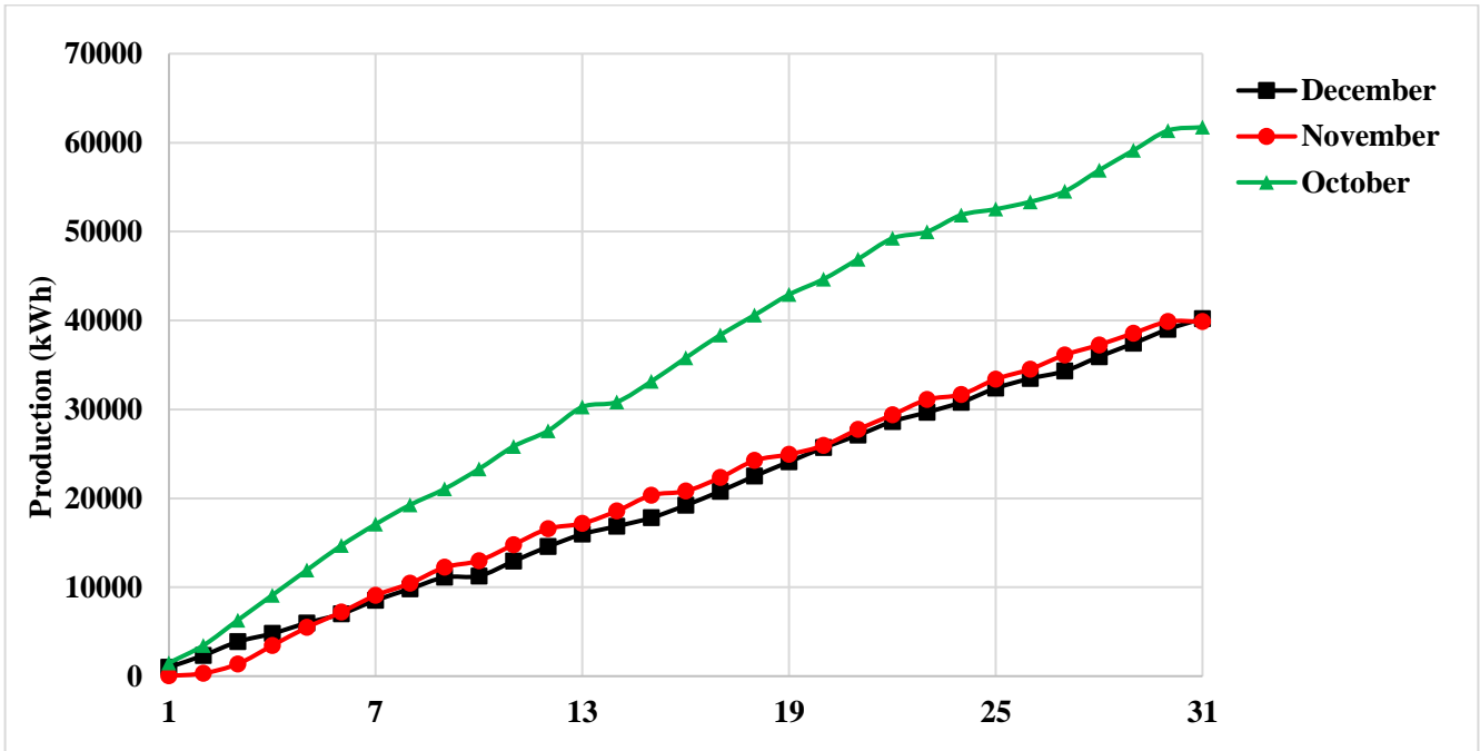
Figure 12.a. Cumulative Daily Production Data for October, November, and December 2021. (Phase-I)
