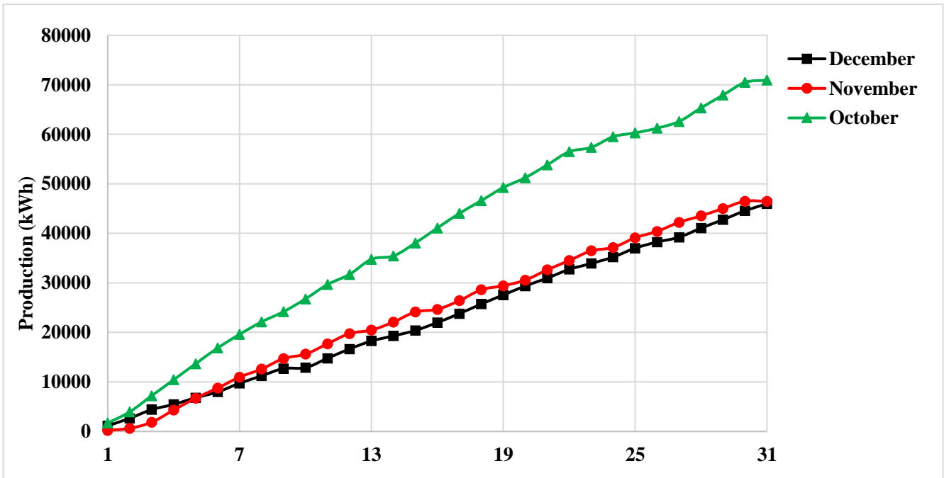
Figure 12.b. Cumulative Daily Production Data for October, November, and December 2021. (Phase-II)
