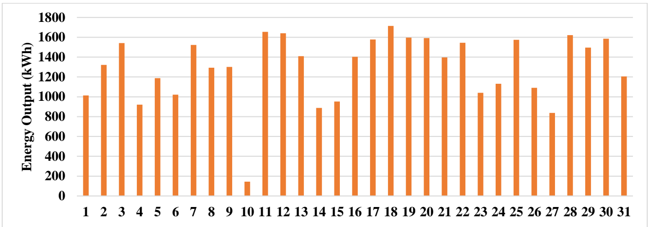
Figure 11.a. Daily Power Output for the Month of December 2021. (Phase-I)
