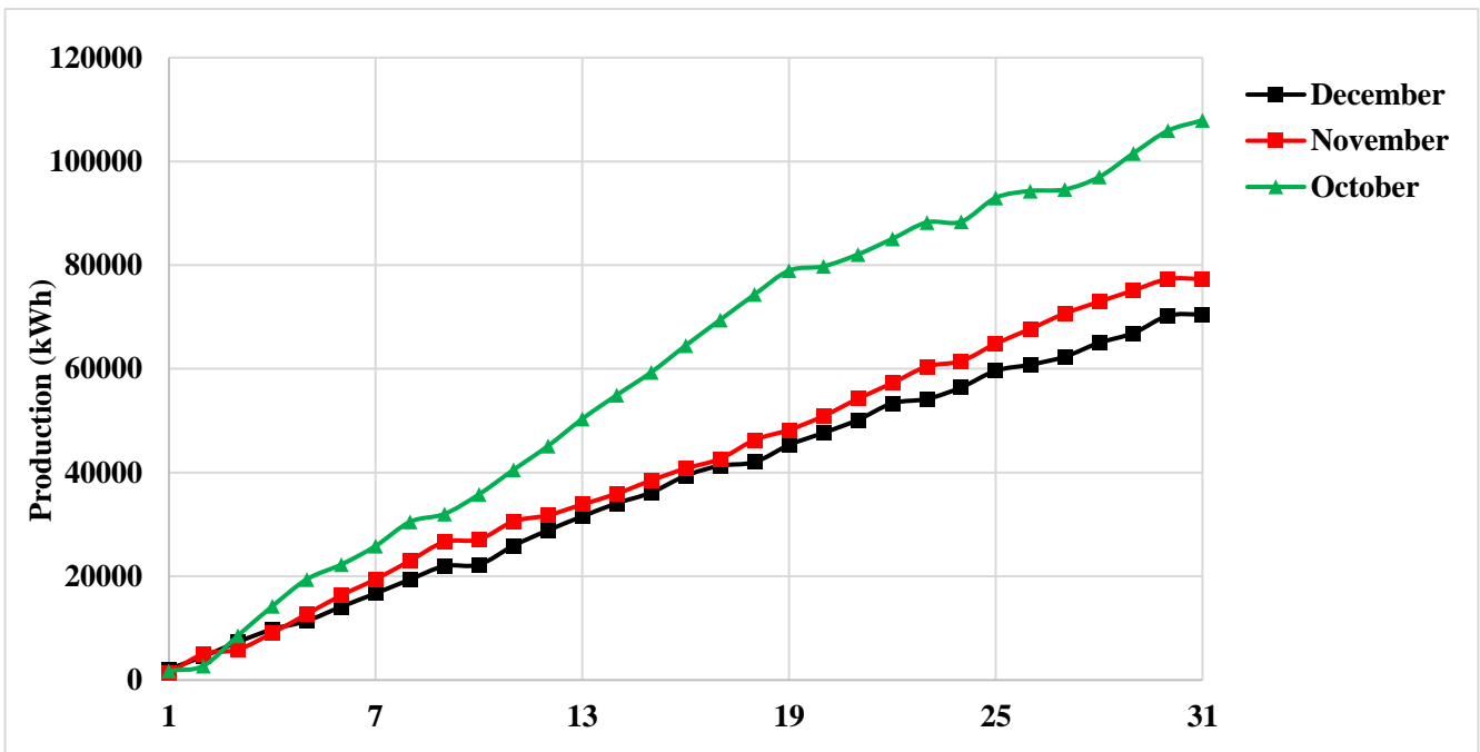
Figure 9. Cumulative Daily Production Data for October, November, and December 2021
