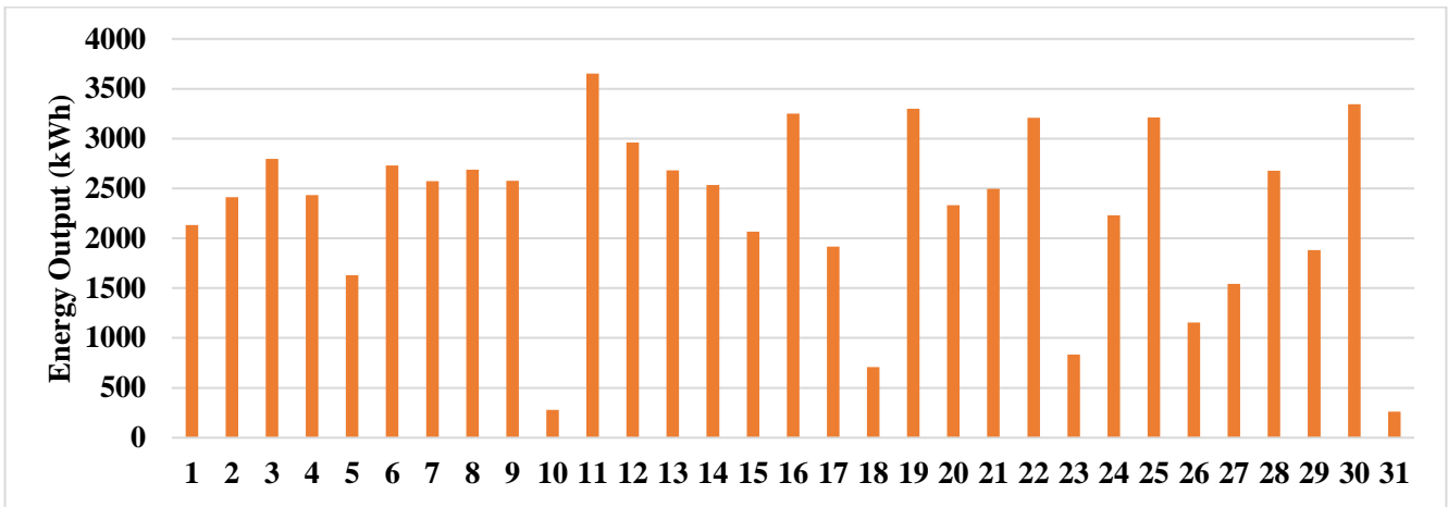
Figure 8. Daily Power Output for the Month of December 2021
