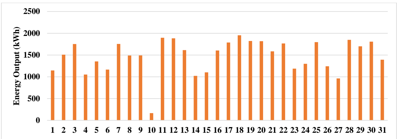
Figure 11.b. Daily Power Output for the Month of December 2021. (Phase-II)
