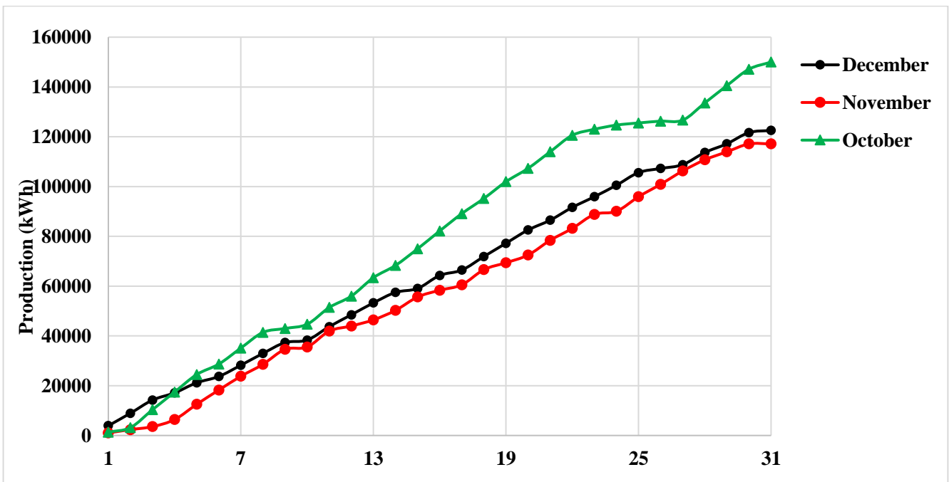
Figure 6. Cumulative Daily Production Data for October, November, and December 2021
