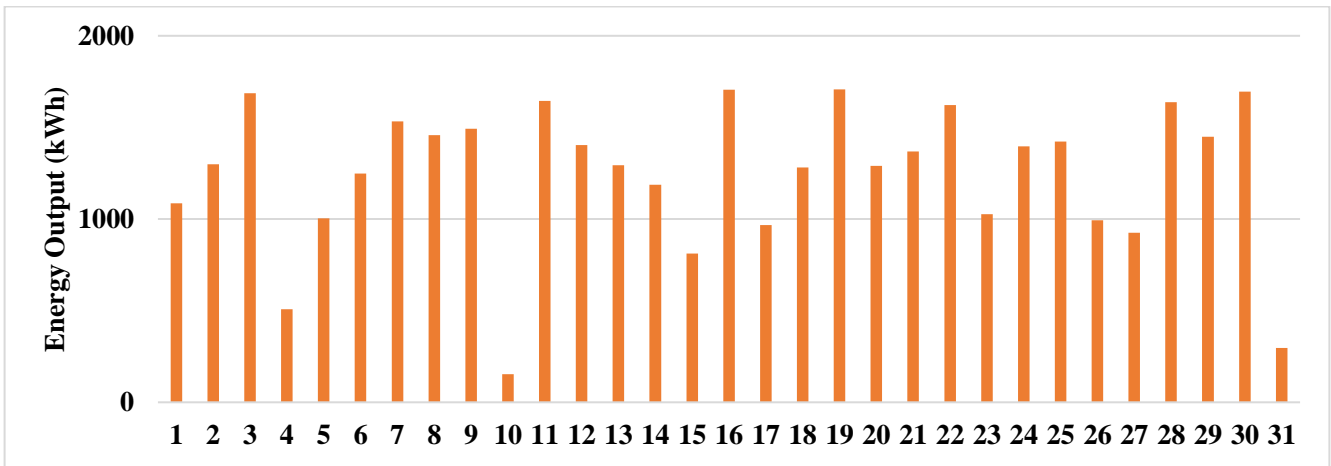
Figure 2. Daily Power Output for the Month of December 2021
