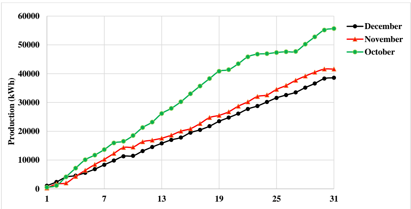
Figure 3. Cumulative Daily Production Data for October, November, and December 2021
