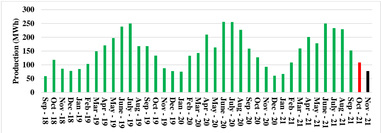
Figure 10. Monthly Production Data for the System since Installation in November 2018
