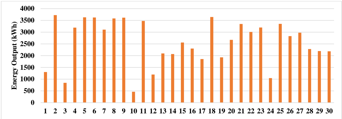
Figure 8. Daily Power Output for the Month of November 2021
