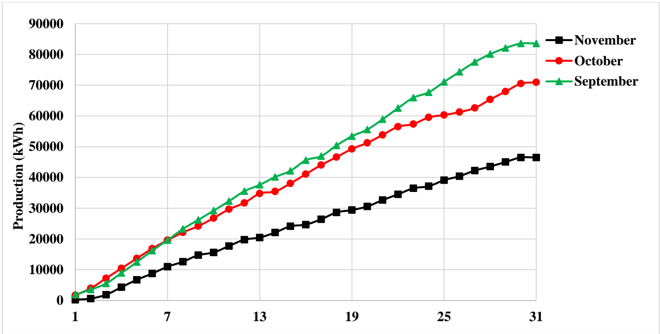
Figure 12.b. Cumulative Daily Production Data for September, October, and November 2021. (Phase-II)
