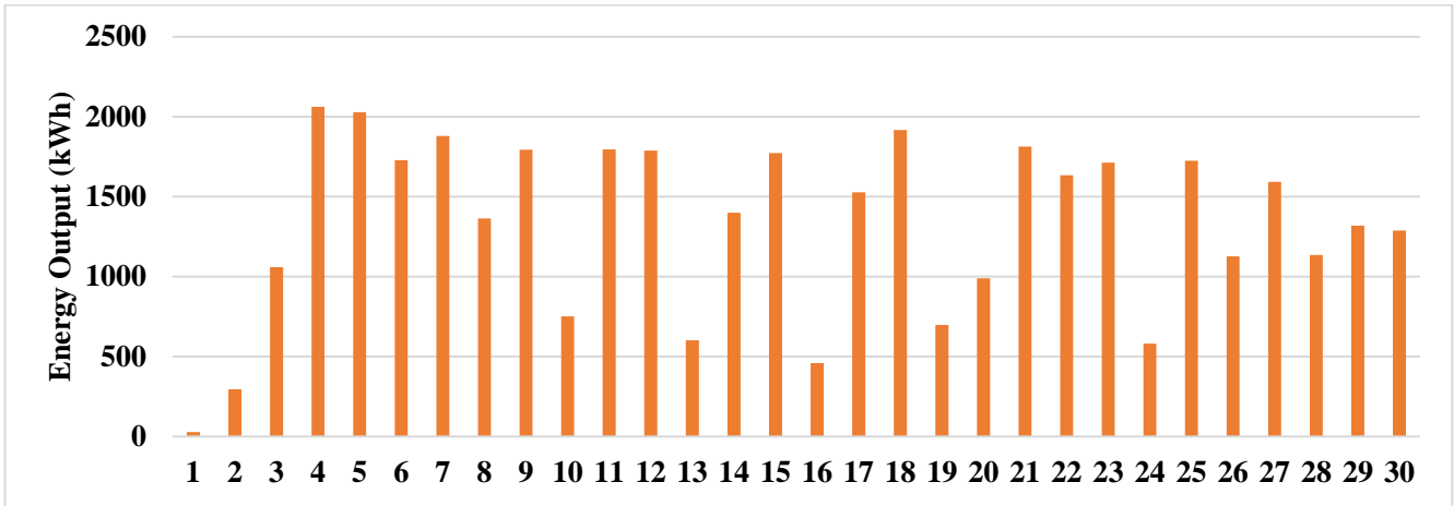
Figure 11.a. Daily Power Output for the Month of November 2021. (Phase-I)
