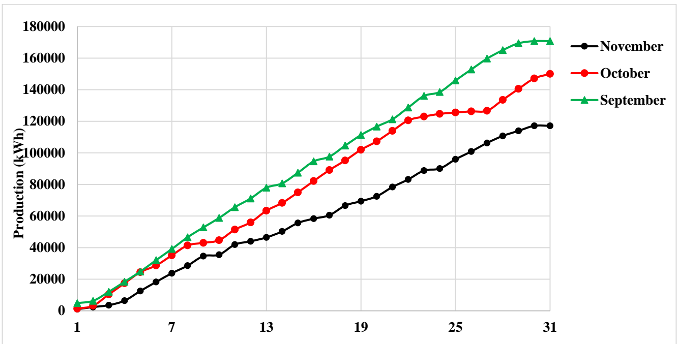
Figure 6. Cumulative Daily Production Data for September, October, and November 2021
