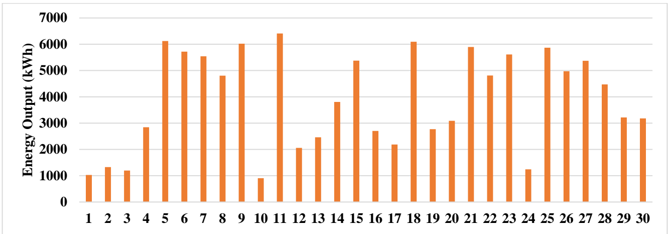
Figure 5. Daily Power Output for the Month of November 2021
