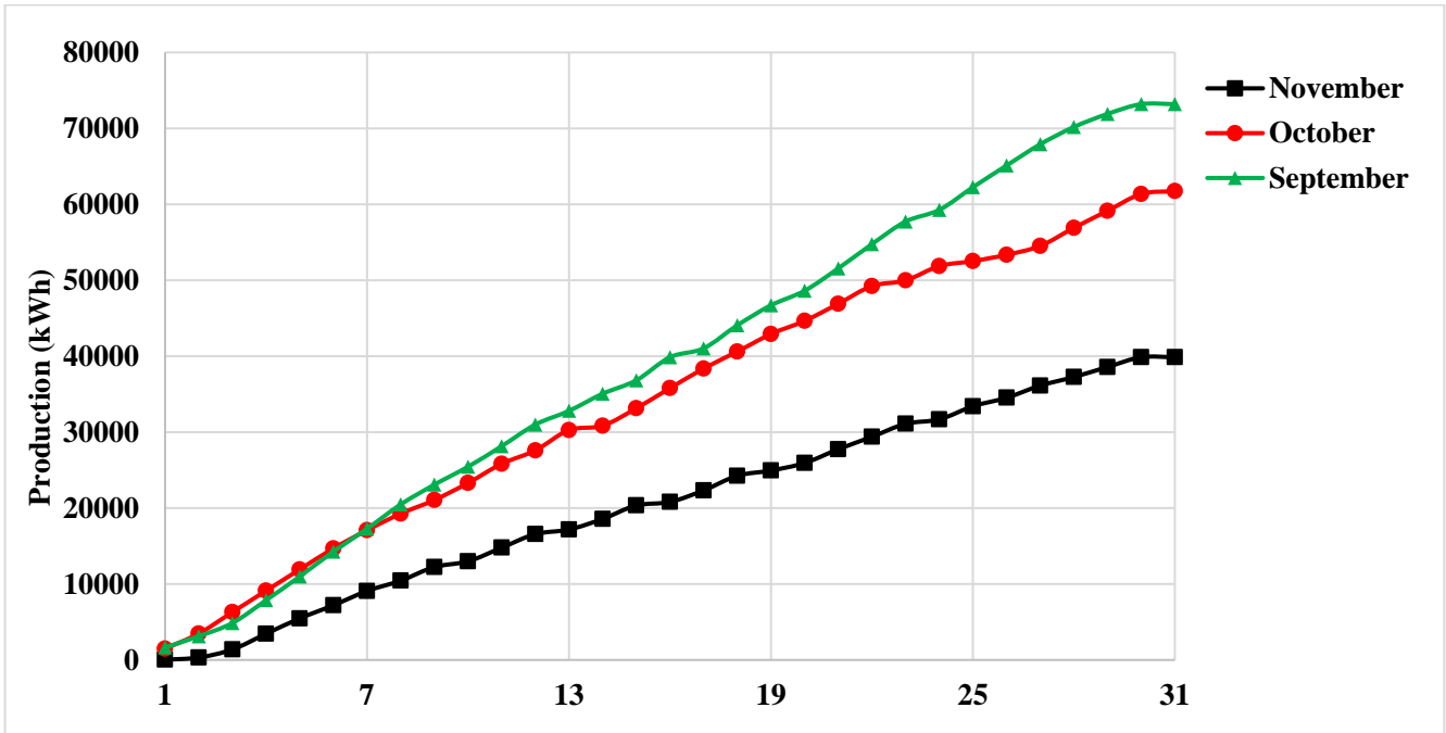
Figure 12.a. Cumulative Daily Production Data for September, October, and November 2021. (Phase-I)
