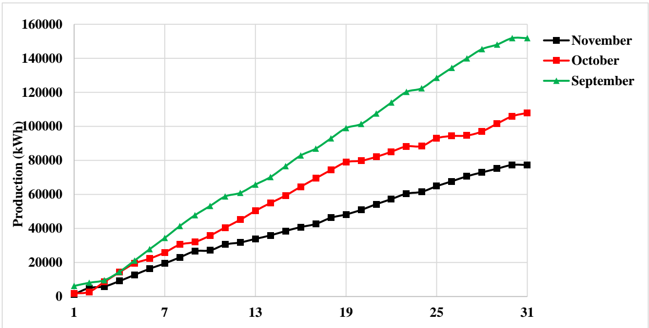
Figure 9. Cumulative Daily Production Data for September, October, and November 2021
