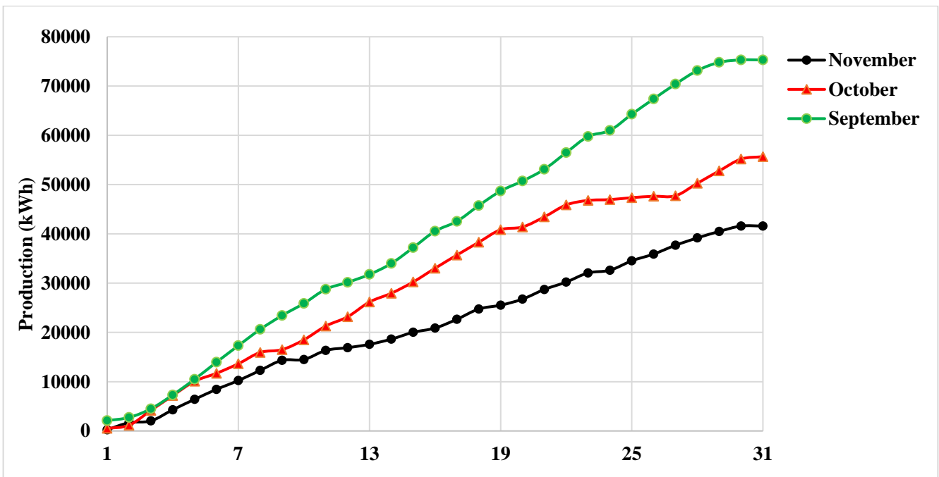
Figure 3. Cumulative Daily Production Data for September, October, and November 2021
