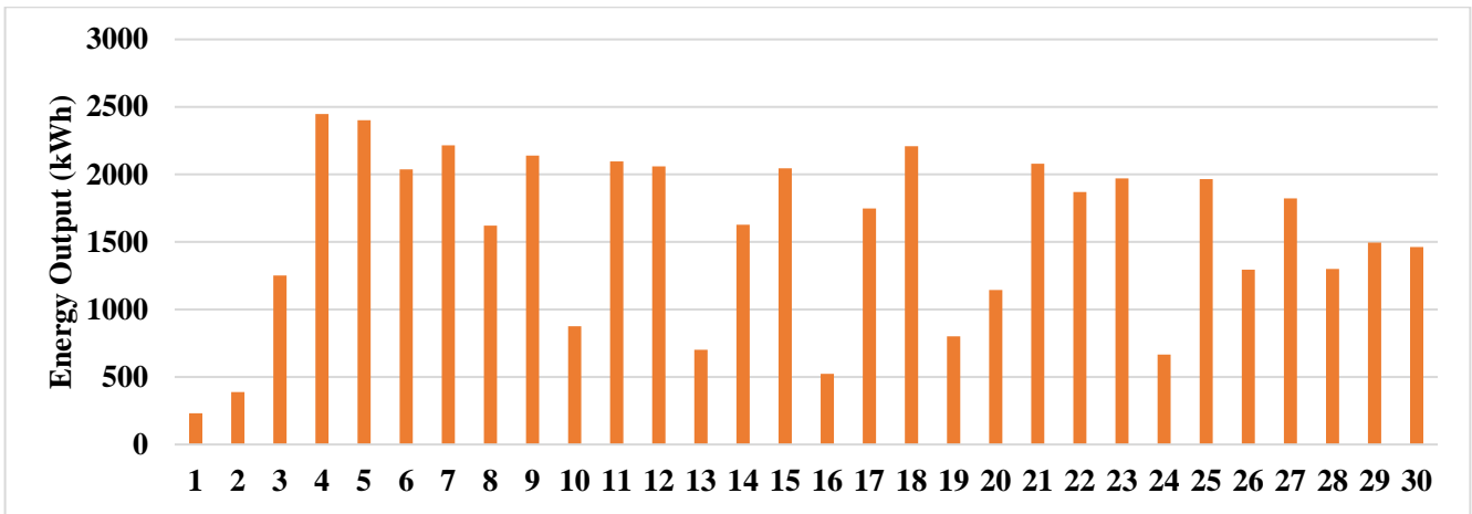
Figure 11.b. Daily Power Output for the Month of November 2021. (Phase-II)
