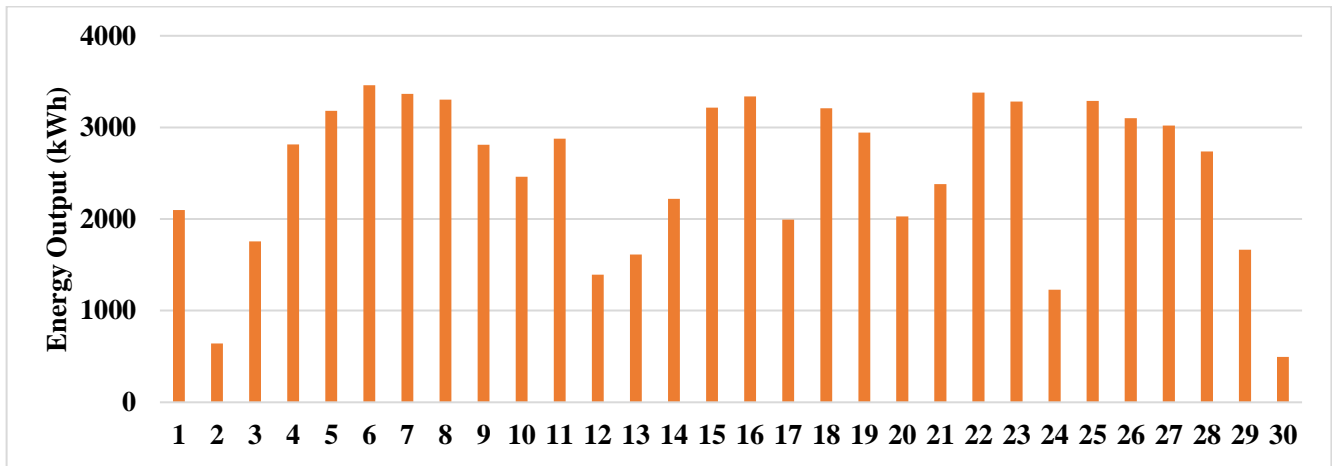
Figure 2. Daily Power Output for the Month of September 2021
