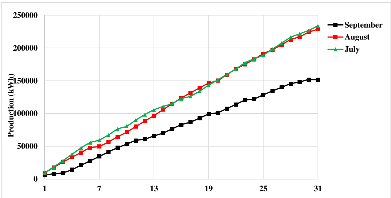
Figure 9. Cumulative Daily Production Data for July, August, and September 2021
