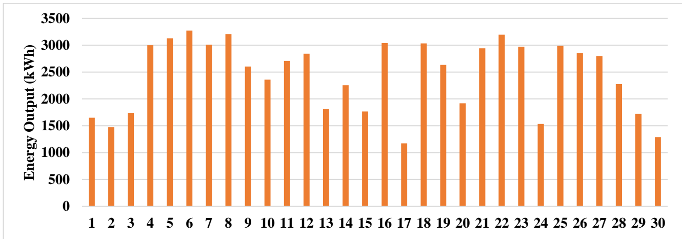
Figure 11.a. Daily Power Output for the Month of September 2021. (Phase-I)*
