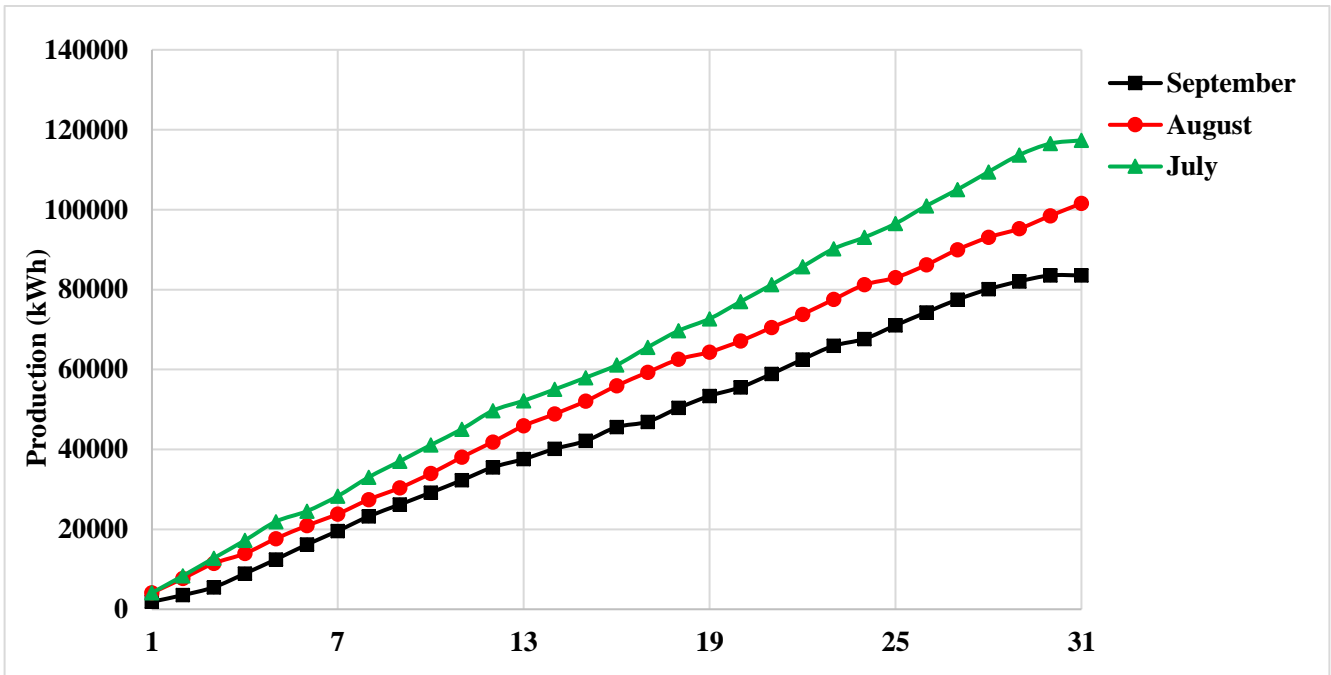
Figure 12.b. Cumulative Daily Production Data for July, August, and September 2021. (Phase-II)
