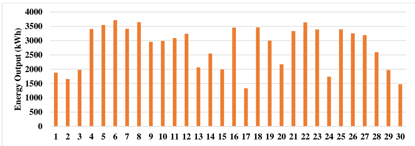
Figure 11.b. Daily Power Output for the Month of September 2021. (Phase-II)
