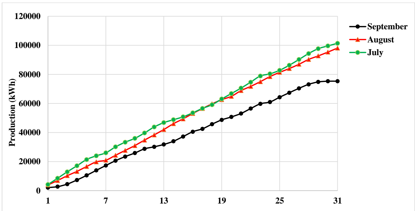
Figure 3. Cumulative Daily Production Data for July, August, and September 2021
