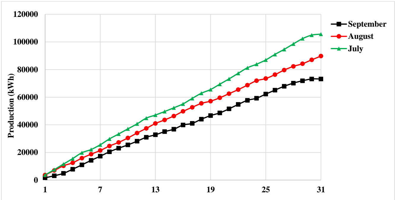
Figure 12.a. Cumulative Daily Production Data for July, August, and September 2021. (Phase-I)
